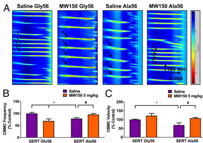
Fig. 3. Repeated administration of a p38 \alpha MAPK inhibitor reverses SERT Ala56-mediated reductions in intestinal motility. (A) Representative spatiotemporal maps showing CMMCs (highlighted by black arrows) in isolated colonic preparations from SERT Gly56 and SERT Ala56 mice administered either saline or MW150 (5 mg/kg, i.p., QD \times 7 d). Ordinate axis represents time and the abscissa represents the distance from oral end to anal end of the resected colon. The width of the gut (millimeters) is pseudo-colored and indicative of contractions. (B) SERT Ala56-mediated reductions in CMMC frequency are normalized by MW150 administration. Data normalized to control (saline SERT Gly56) ( n = 8-12 per group, two-way ANOVA, followed by post hoc Fisher's LSD multiple comparison tests, F_{1, 60} = 17.12 , *P \leq 0.01 , saline SERT Gly56 vs. saline SERT Ala56 and saline SERT Gly56 vs. MW150 SERT Gly56, \#P \leq 0.05 MW150 SERT Ala56 vs. saline SERT Ala56). (C) SERT Ala56-mediated reductions in CMMC velocity are normalized by MW150 administration. Data normalized to control (saline SERT Gly56) ( n = 8-12 per group, two-way ANOVA, followed by post hoc Fisher's least-significant difference multiple comparison tests, F_{1, 60} = 10.47 and 14.19 , *P \leq 0.05 , saline SERT Gly56 vs. saline SERT Ala56, \#P \leq 0.05 MW150 SERT Ala56 vs. saline SERT Ala56).
